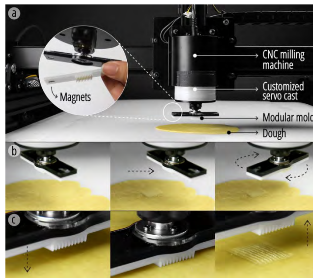
Figure 12: Digital fabrication for the grooving process. (a) A CNC machine was equipped with a rotational tool head with a replaceable grooving mold. (b) The tool head goes through a cycle of rotating and grooving according to the design. (c) The result of the automatic grooving.
