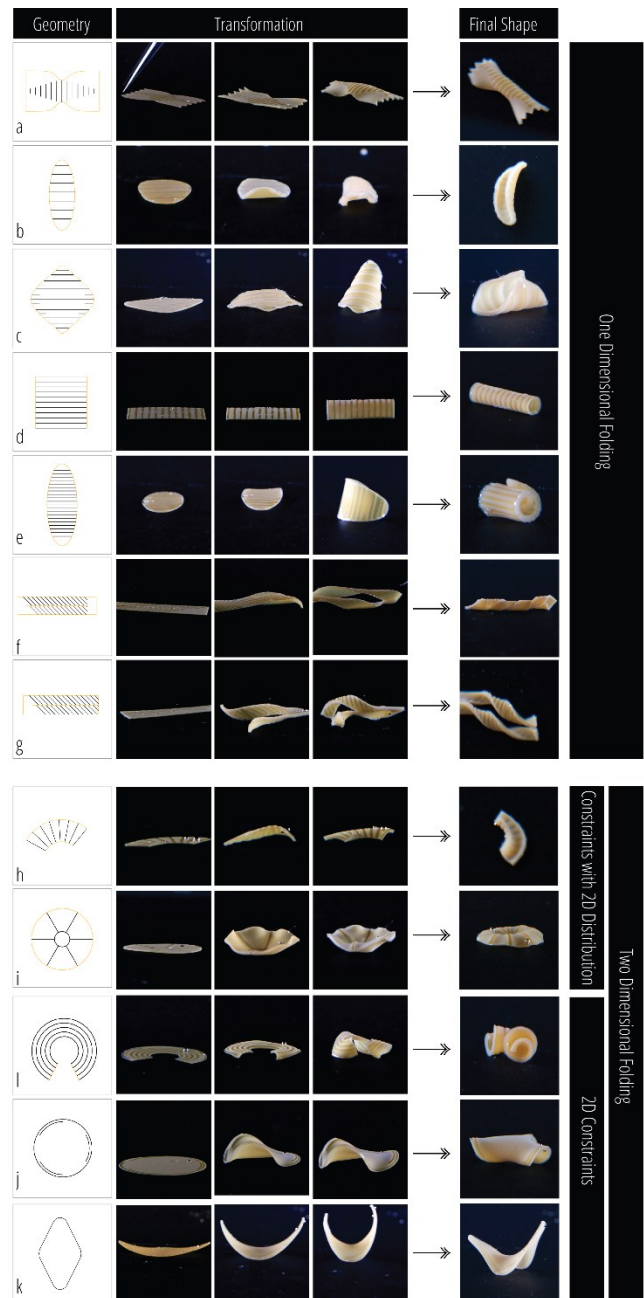
Figure 13. Folding Algorithm.
