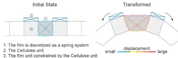
Figure 10. Simulation model units.
