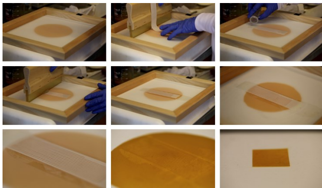
Figure 12. Screen printing process.
