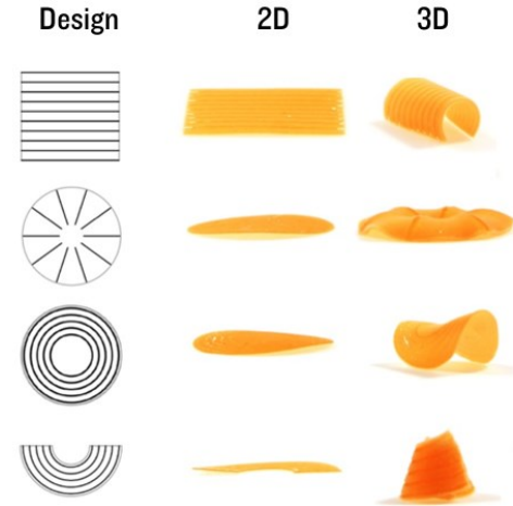
Figure 8. Design primitives (black lines indicate fiber location).
